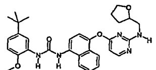
1-(5-tert-Butyl-2-methoxy-phenyl)-3-(4-{2-[(tetrahydro-furan-2-ylmethyl)-amino]-pyrimidin-4-yloxy}-naphthalen-1-yl)-urea;
